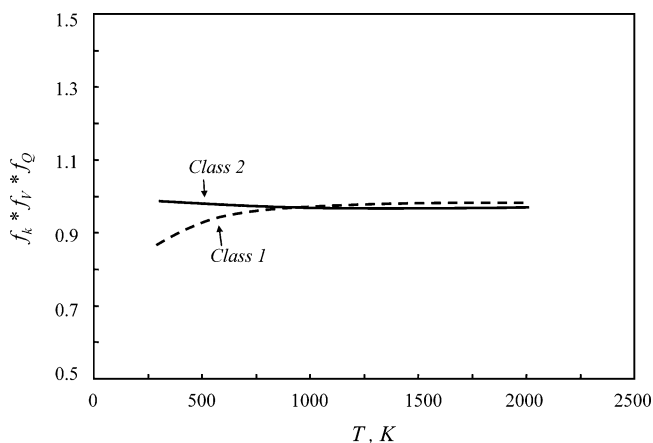
Figure 6. Relative rate factor f'(T) = f_Q f_k f_v for Class 1 and Class 2.
